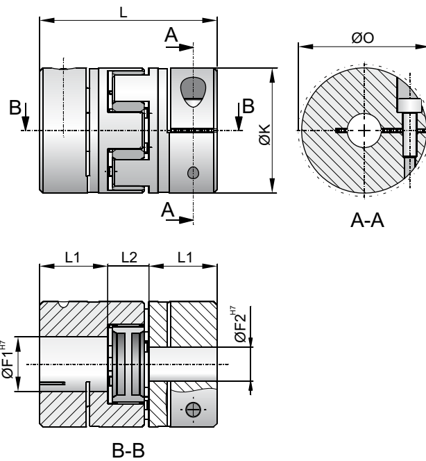
Dimension table - motor coupling HMRS
