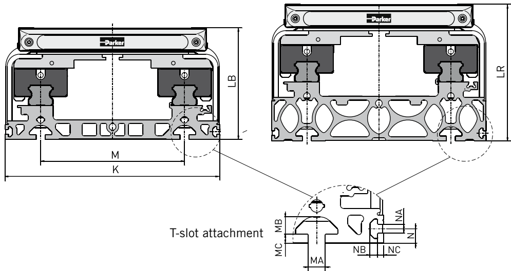
“Reinforced” profile
